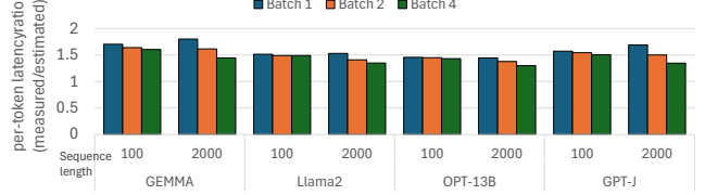
Fig. 8: Measured vs. modeled average per-token decoding latencies for four LLM models on A100 for sequence lengths of 100 and 2000 tokens and a 200-token input.
